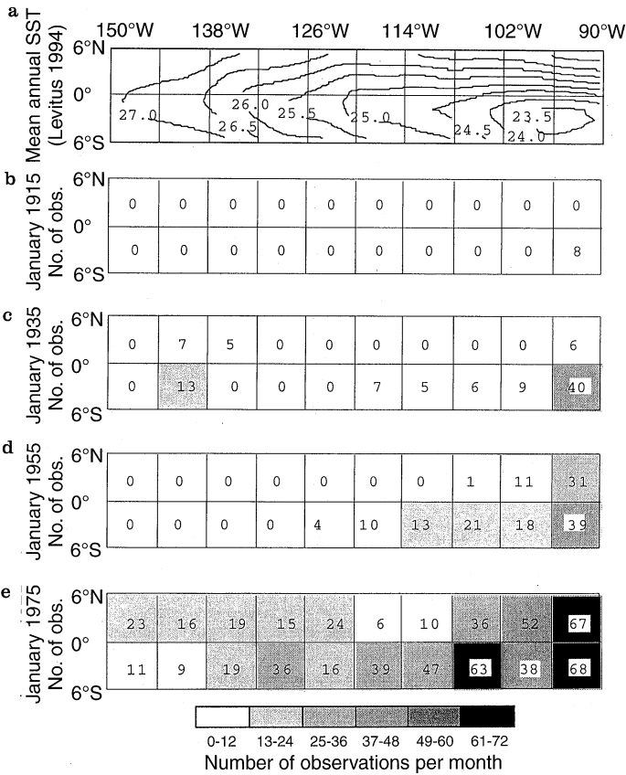
Fig. 2a–e. Observational frequency in the Niño-3 region. a Mean annual sea surface temperature (Extended to 6°S–6°N to accommodate data gridded in 2° × 2° boxes, Levitus 1994). b, c, d, e Observational frequency for January 1915, January 1935, January 1955, and January 1975, respectively
