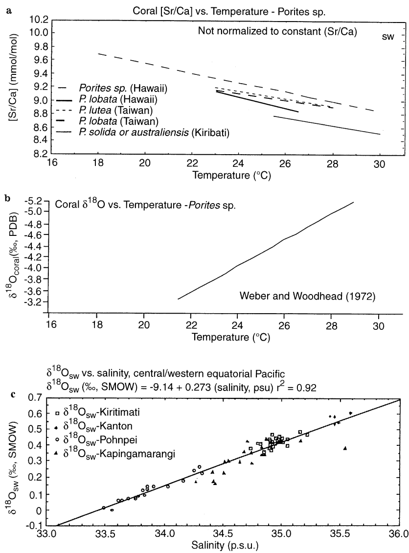
Fig. 4a–c. Tracers of sea surface temperature and salinity. a Sr/Ca vs. SST for several species of Porites (Schneider and Smith 1982; De Villiers et al. 1994; Shen et al. 1996; Evans et al. submitted 1997). b \delta^{18}\text{O}_{\text{coral}} vs. SST for Porites sp. The slope is 0.22\text{‰}\delta^{18}\text{O}/^{\circ}\text{C} . c \delta^{18}\text{O}_{\text{seawater}} vs. sea surface salinity for the central and western Pacific (data from this work)
