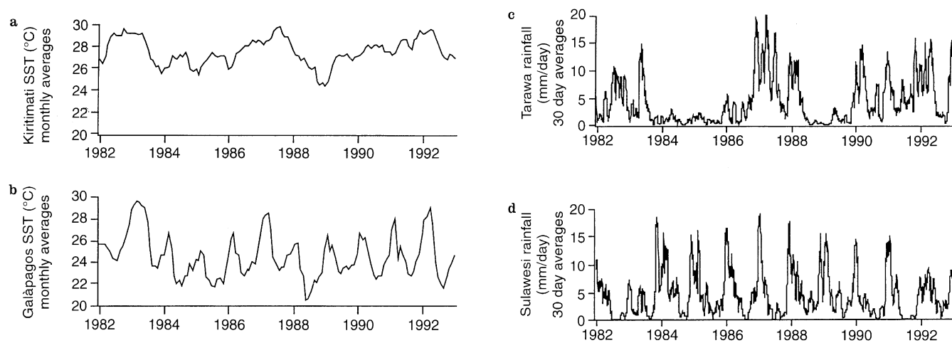
Fig. 6a-d. The seasonal cycle of sea surface temperature and rainfall at four sites spanning the equatorial Pacific. Interannual variations are manifestations of ENSO. a SST at Kiritimati; b SST at Galapagos; c rainfall at Tarawa; d rainfall at Sulawesi. Data from Reynolds and Smith (1994) and Spencer (1993)
