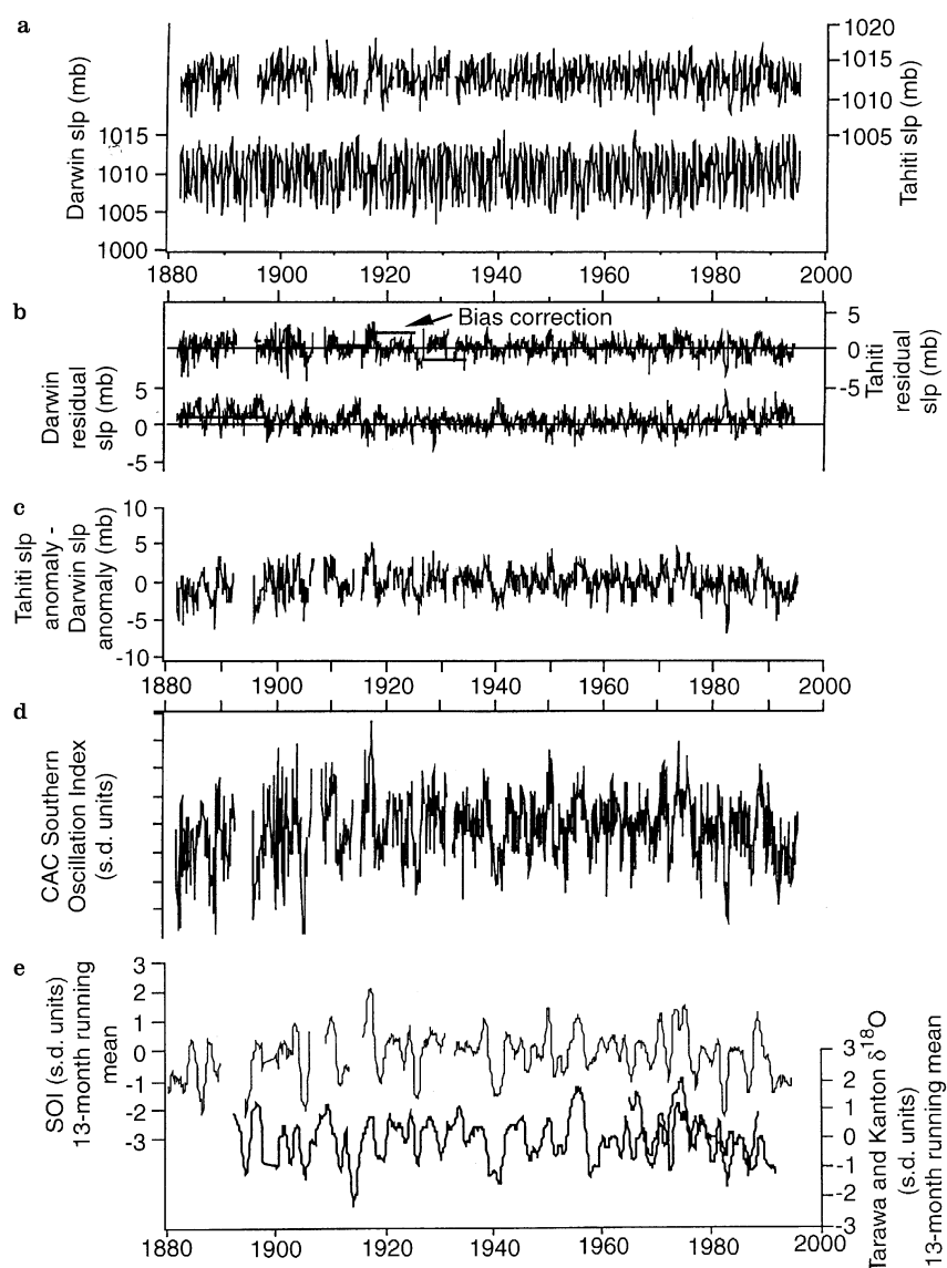
Fig. 3a–e. Construction of the Southern Oscillation Index and comparison with coral data from Tarawa Atoll and Kanton Island. a Raw sea level pressure data; b sea level pressure anomaly series, before bias corrections; c differenced anomaly series; d standardized SOI (Climate Analysis Center 1996); e SOI ( top curve ) and coral time series (Tarawa record is 1894–1989, Kanton is 1965–1992), smoothed with a 13-month box filter
