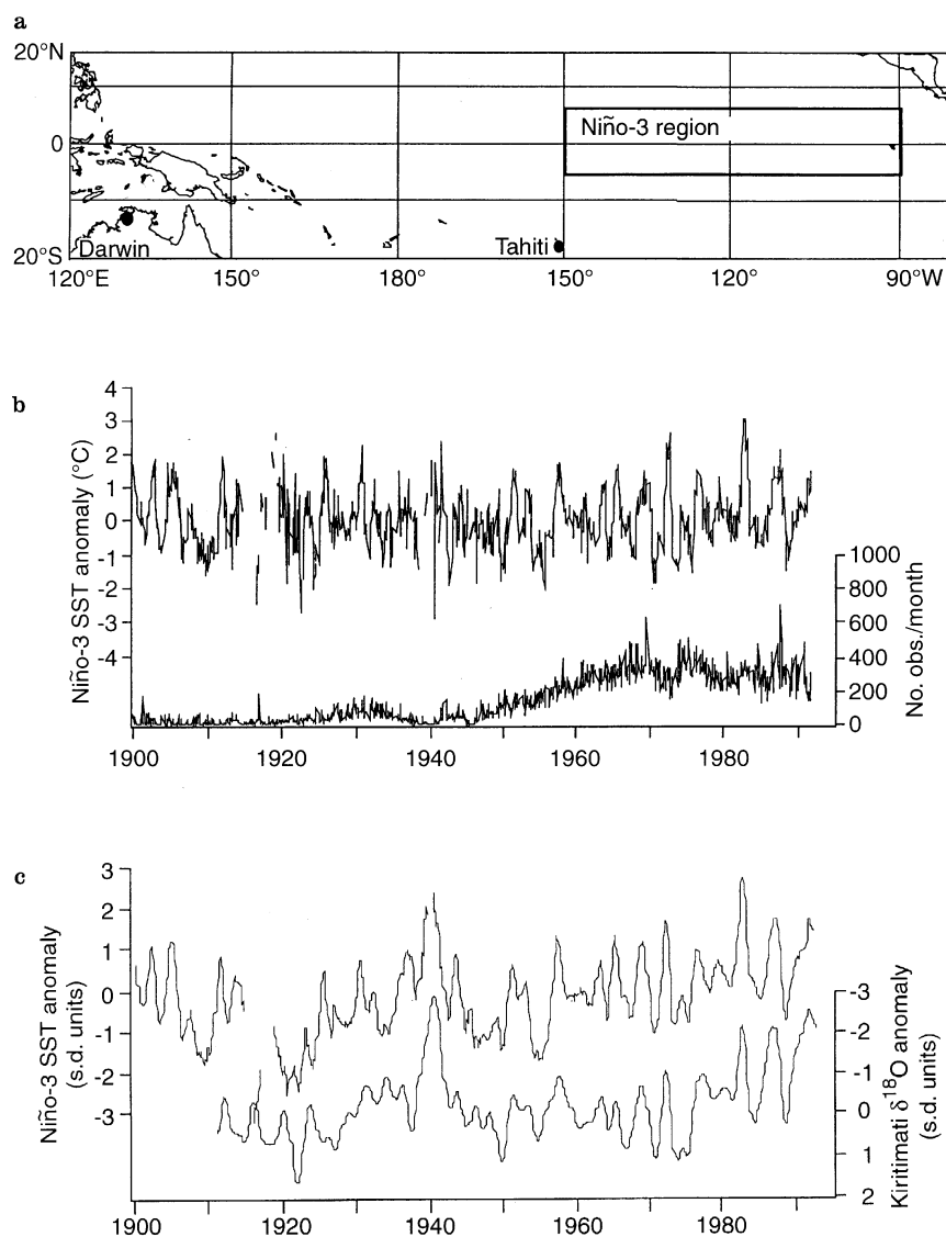
Fig. 1a–c. Construction of the Niño-3 SST anomaly index, and comparison with coral data from Kiritimati. a Geographic extent of the Niño-3 box. b Niño-3 SST anomaly and number of observations per month (from GOSTA data; Bottomley et al. 1990). c Niño-3 SST anomaly compared to the Kiritimati anomaly series, smoothed with a 13-month box filter
